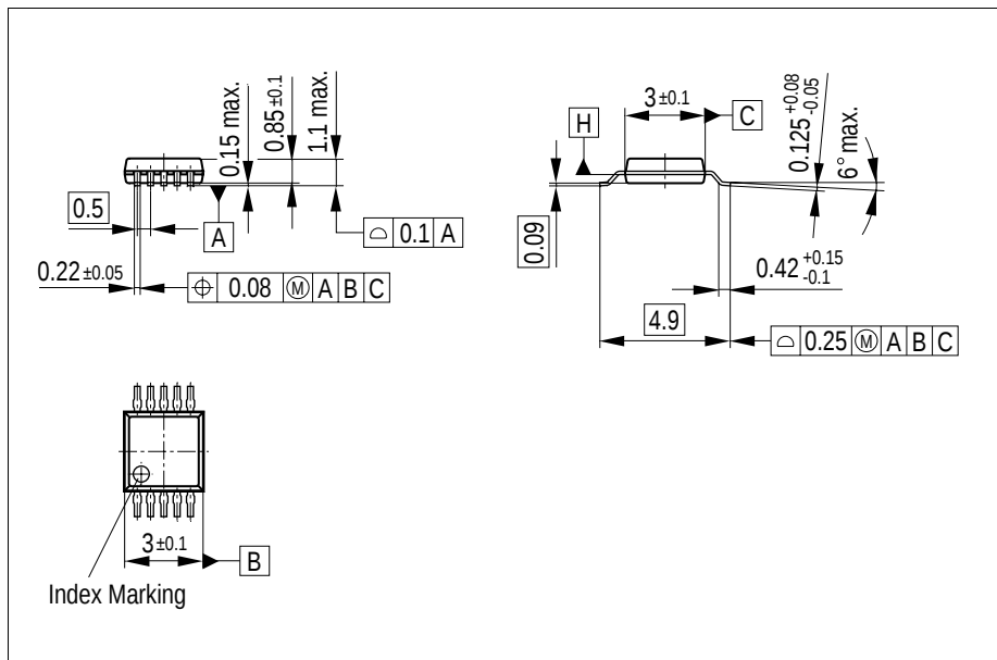
Figure 18 PG-TSSOP-10
